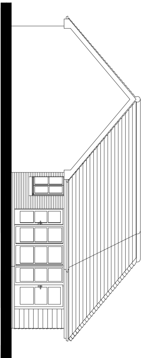
BUNGALOW - REAR LEFT ELEVATION
